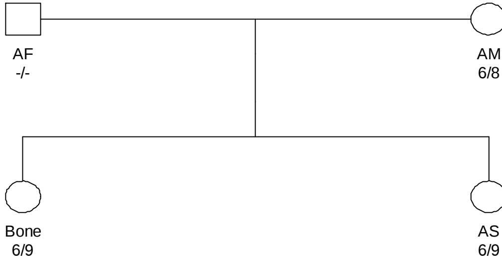
Figure 3. CAP paper challenge. Marker F13B. Frequencies: 6:0.086, 8:0.152, 9:0.328, rest:0.434
