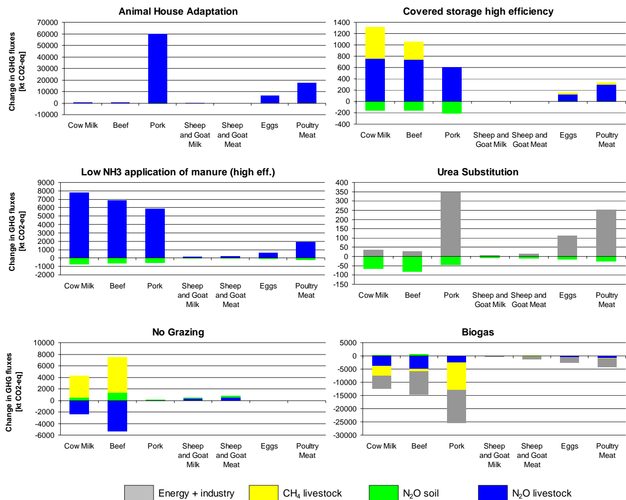
Figure ES11. Impact of selected technological abatement measures, compared with the reference situation for the year 2004, if the measure would be applied by all farms, calculated with a cradle-to-gate life-cycle analysis with CAPRI
