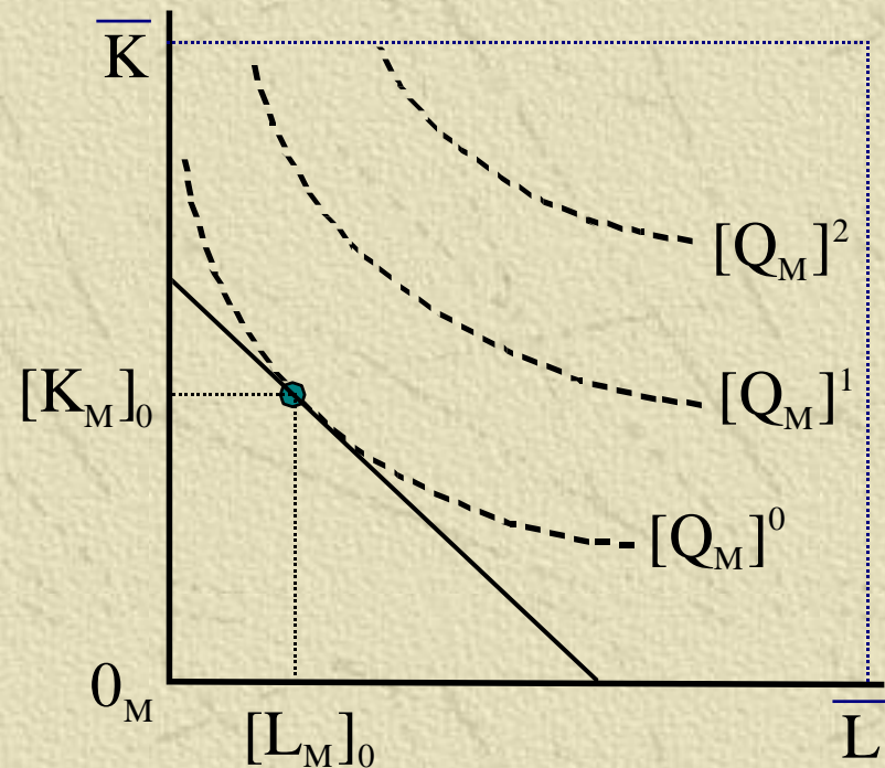
Manufacturing sector
