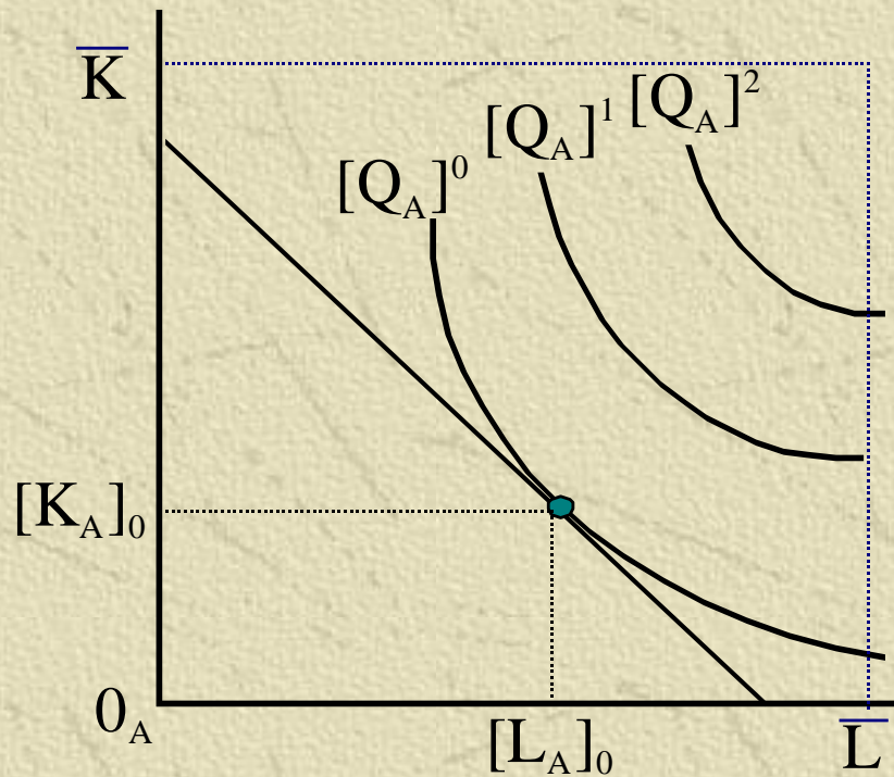
Agricultural sector
